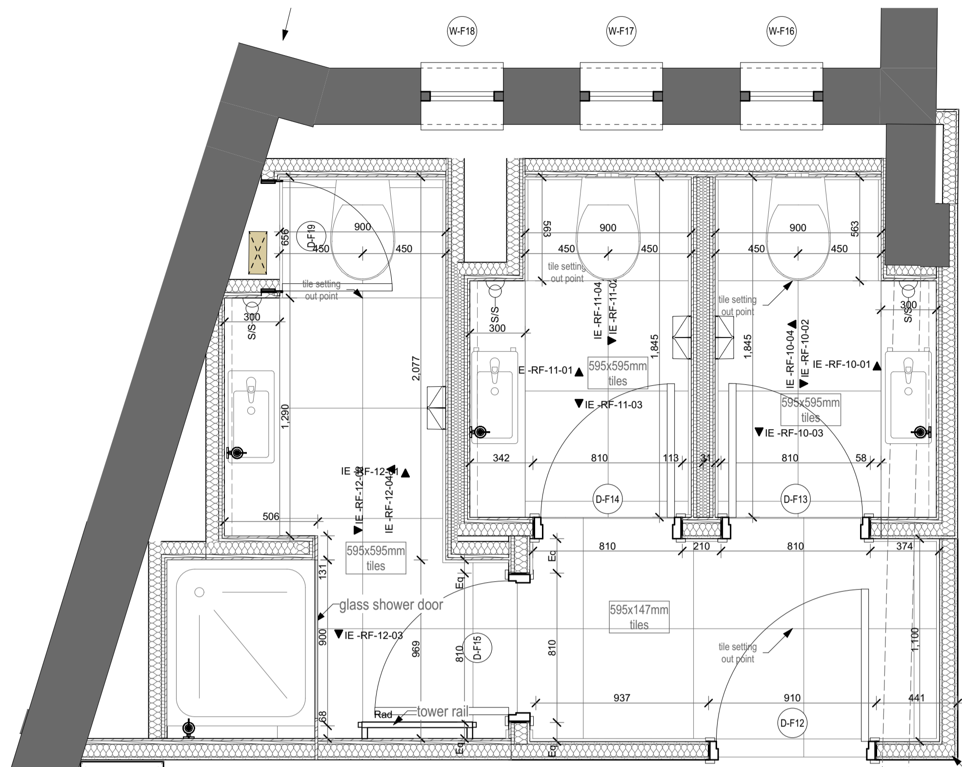
1 Fourth Floor: 1:20 GA's
