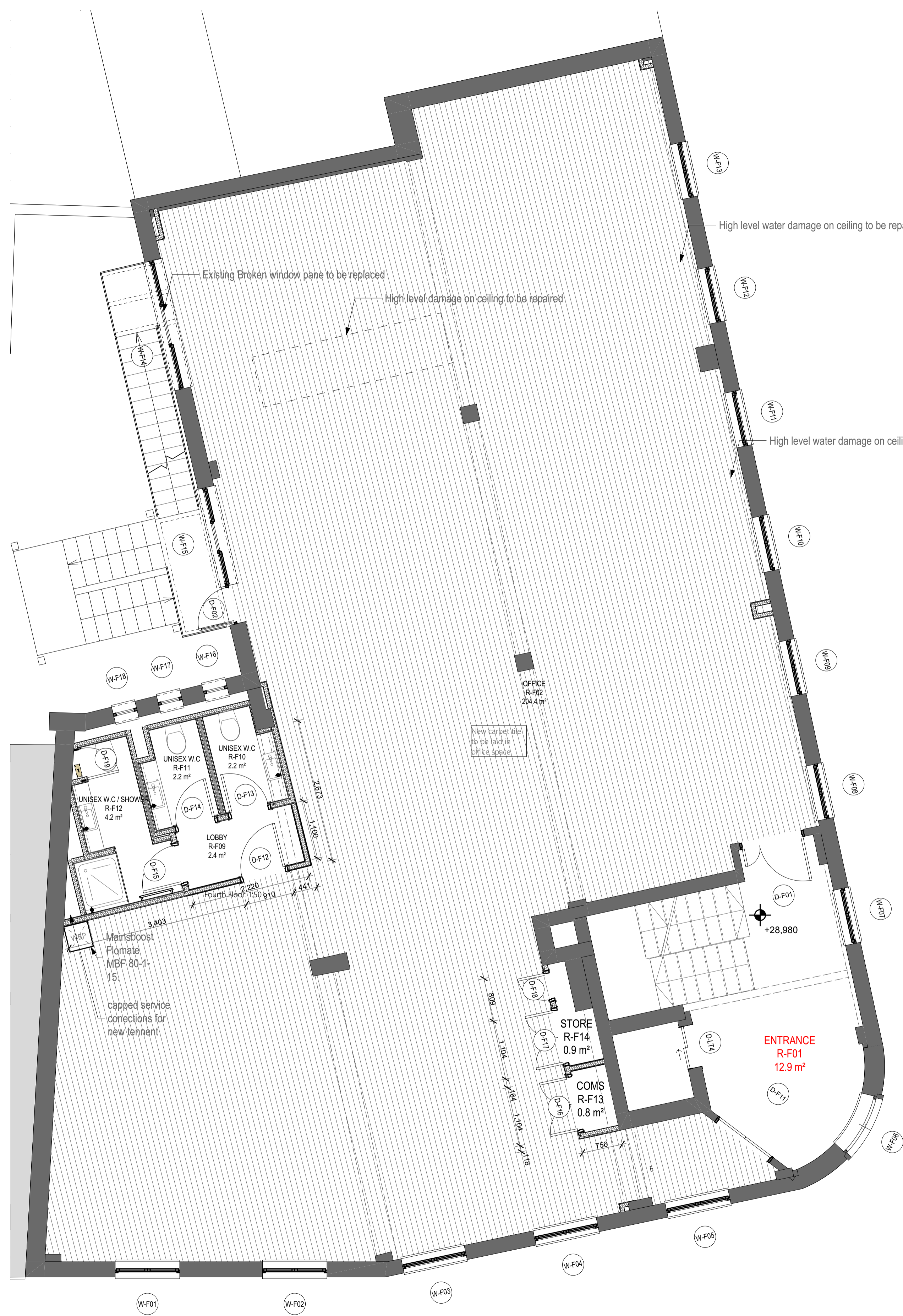
2 Fourth Floor: 1:50 GA's
